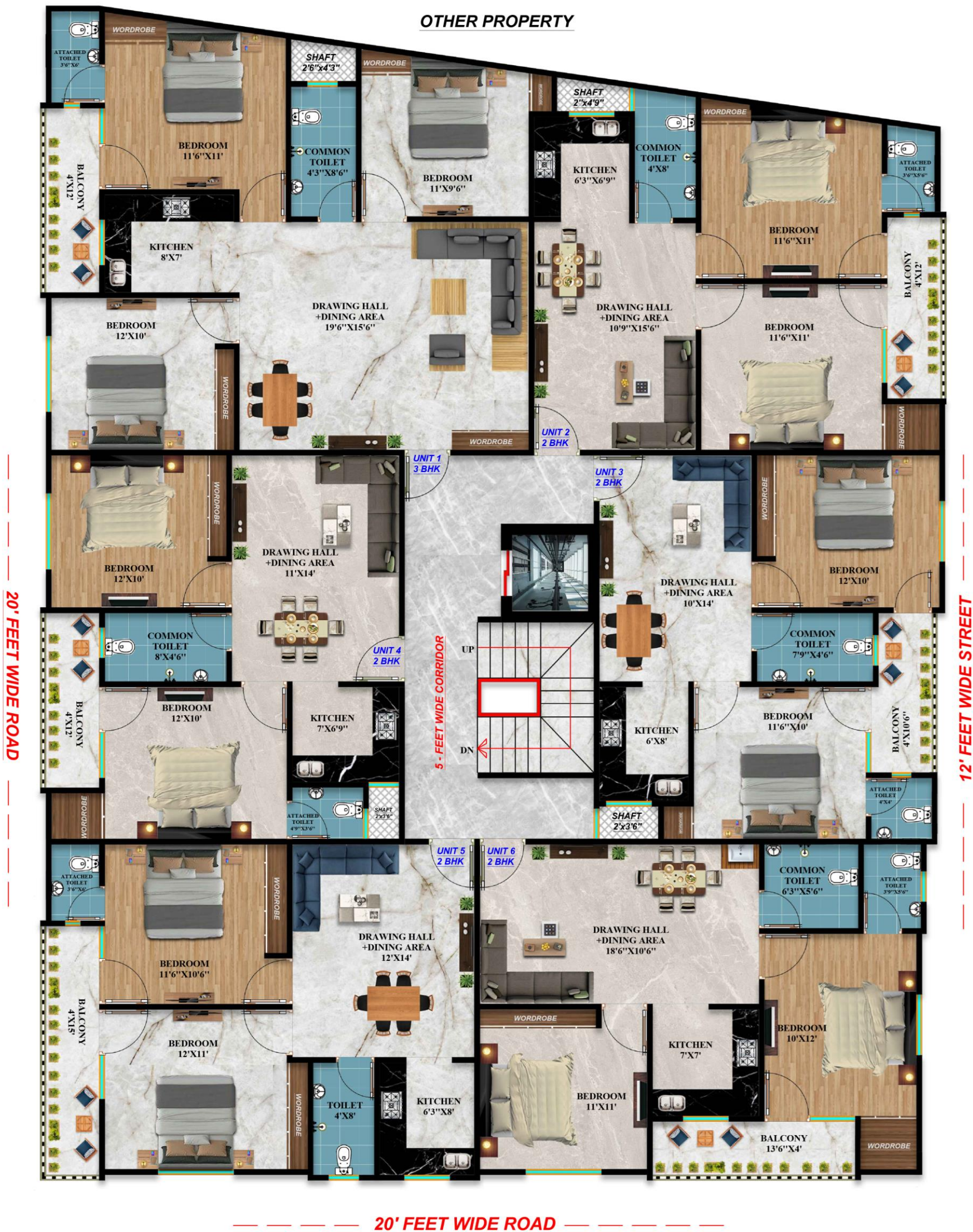
TYPICAL FLOOR FINAL FURNITURE LAYOUT
